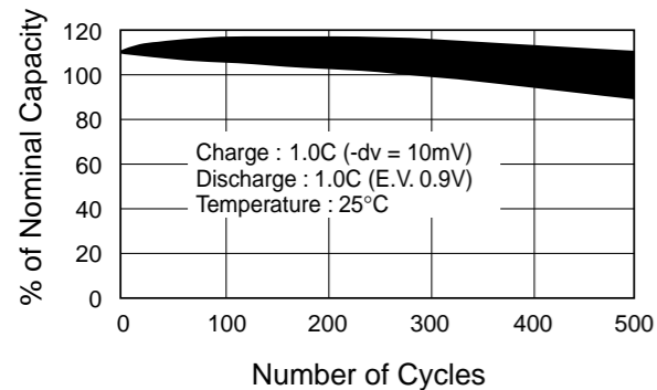
Charge/Discharge Cycle Characteristics
